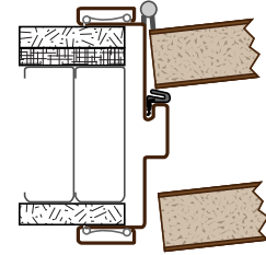
3C Jamb Hinge/Strike - Kerfed
