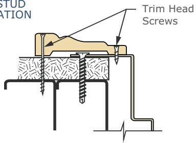
WOOD STUD APPLICATION
