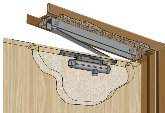
LCN 3130 Concealed in the door
