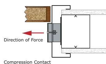
16 or 18 Ga. Drywall Frame - Knocked Down
