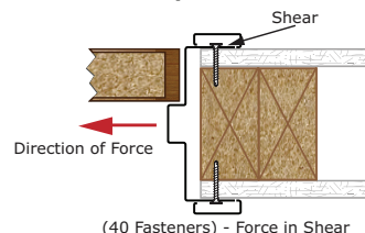
20 Ga. Prefinished Drywall Frame - Knocked Down (KD)
