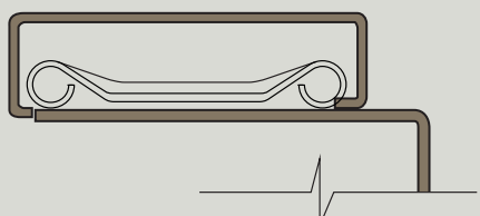
TA-23 Aluminum Casing
