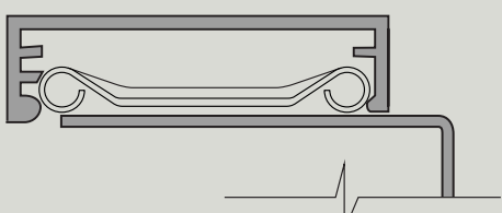
TA-28 Aluminum Casing
