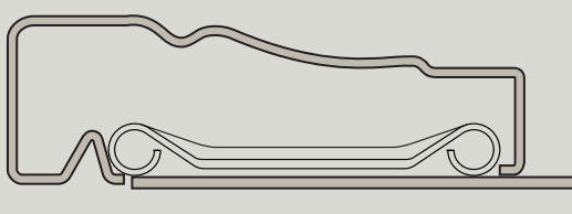
TA-30 Colonial Steel Casing
