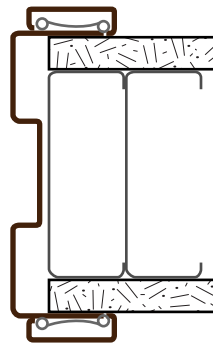
6V Jamb - Inverted Stop
