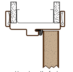
3D Header - Kerfed
