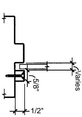
6 Glass Stop (TA14)
