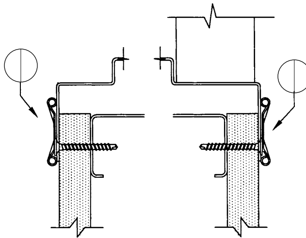
6 Split Casing Design
